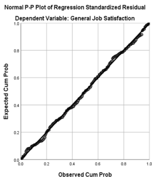
Figure 3. Normal Probability Plot for General Job Satisfaction
