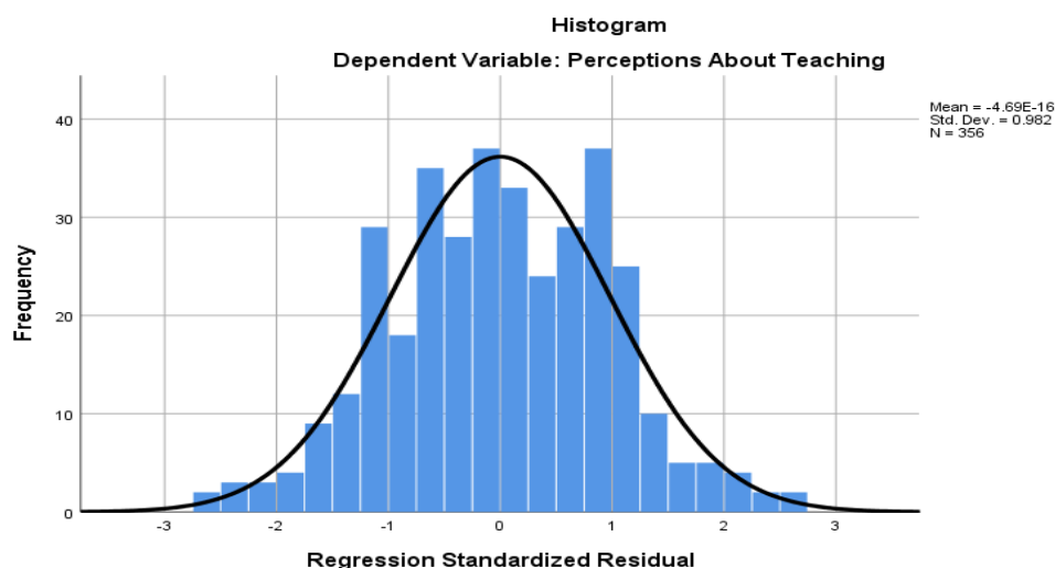
Figure 4. Histogram of Standardized Residuals for Teacher Perceptions
