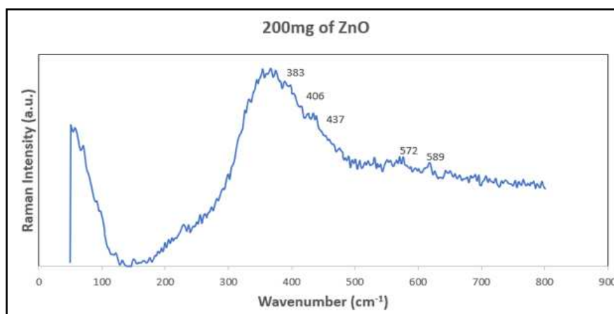
Figure 6. Raman spectra of the 200 mg ZnO film (sample 3).
