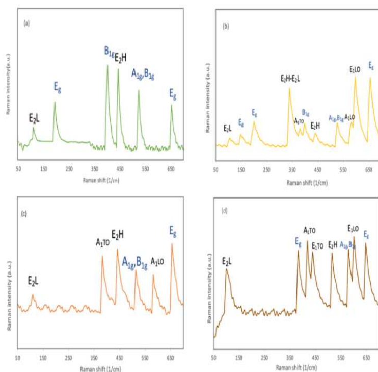
Figure .7 Raman spectra images of (a) one-layer, (b) two-layers, (c) three-layers, and (d) four-layers of ZnO/ \text{TiO}_2 films.
