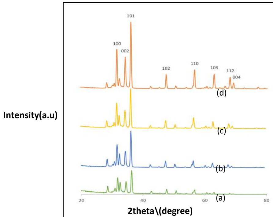
Figure 1. X-ray diffraction patterns for doped polyethylene , and dopped with (a) 100 mg ,(b) 150 mg,(c) 200 mg , and (d) 250 mg of ZnO powder.
